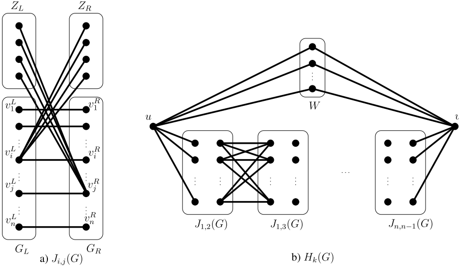
Fig. 3. The construction of J_{i,j} (a) and H_k(G) (b).
