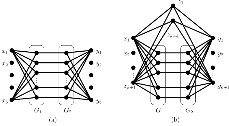
Fig. 2. The construction of G' for k = 4 (a) and for k \geq 5 (b).
