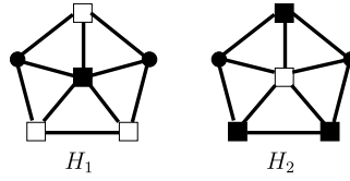
Fig. 1. The placement of the vertices of H_1 and H_2 in U_1 and U_2 ; the vertices denoted by black squares are in U_1 and the vertices denoted by white squares are in U_2 .
