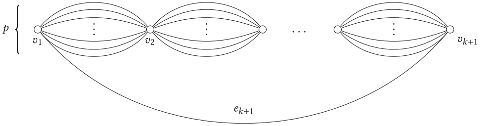
Fig. 1. Construction of the multigraph G(k, p) .
